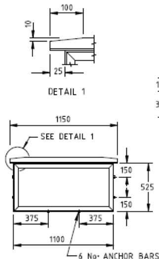
GRATE FRAME
