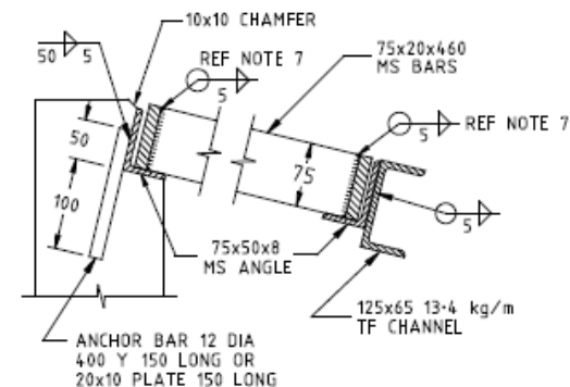
SECTION THROUGH GRATE
