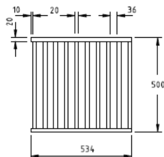
GRATE
